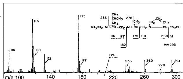
Fig. 2. Mass spectrum of the derivative of a tripeptide (Leu Ala Pro) (Reprinted from Ref. [3] with permission from Elsevier).
